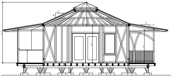
1 BUILDING SECTION Scale: 3/16" = 1'-0"
